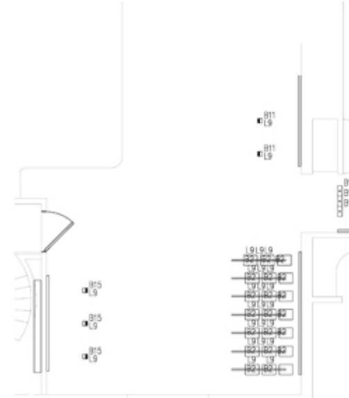
WEST ART ROOM SCALE: 1/4" = 1'-0"
