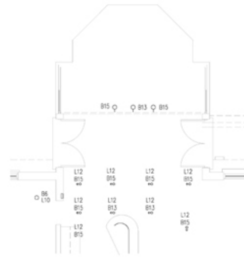
SOUTH SUN ROOM SCALE: 1/4" = 1'-0"
