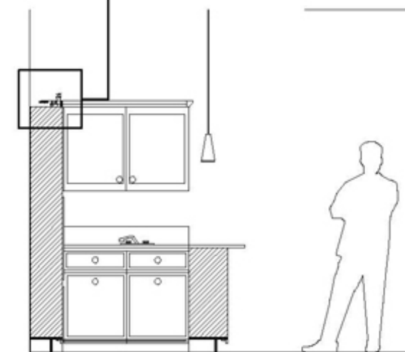
DT3 DETAIL OF FLUORESCENT UP DISPLAY SCALE: 1/4" = 1' - 0"
