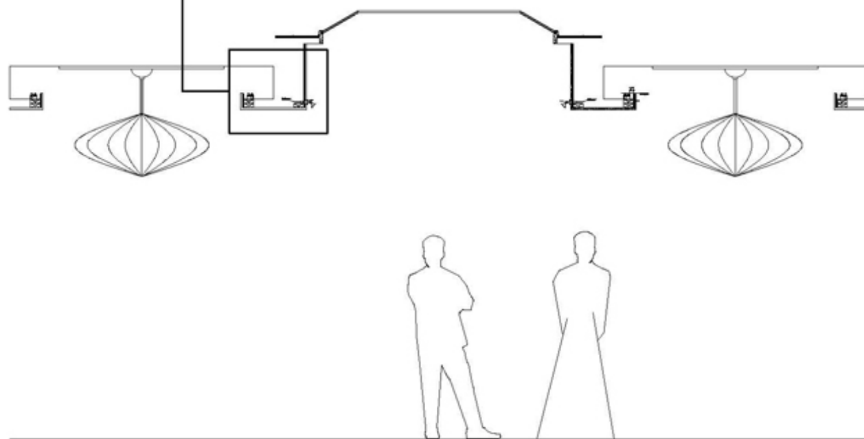
DT1 DETAIL OF FLUORESCENT COVE DISPLAY SCALE: 1/4" = 1' - 0"
