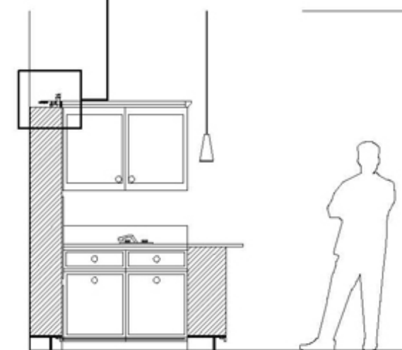
DT3 DETAIL OF FLUORESCENT UP DISPLAY SCALE: 1/4" = 1' - 0"
